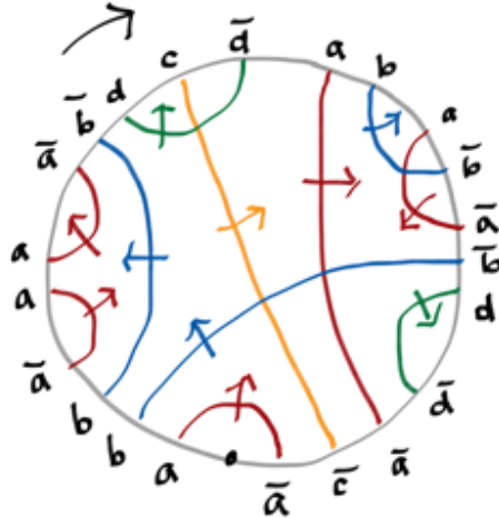
FIGURE 1. Disk diagram for the identity word abb̄aāb̄d̄cd̄abab̄āb̄d̄d̄āc̄ā , where \bar{x} is the inverse of x .
